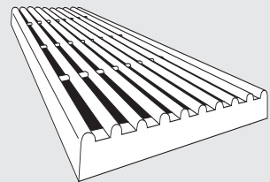
Concrete Cattle Guard 1' 4" L x 6' 5" W
